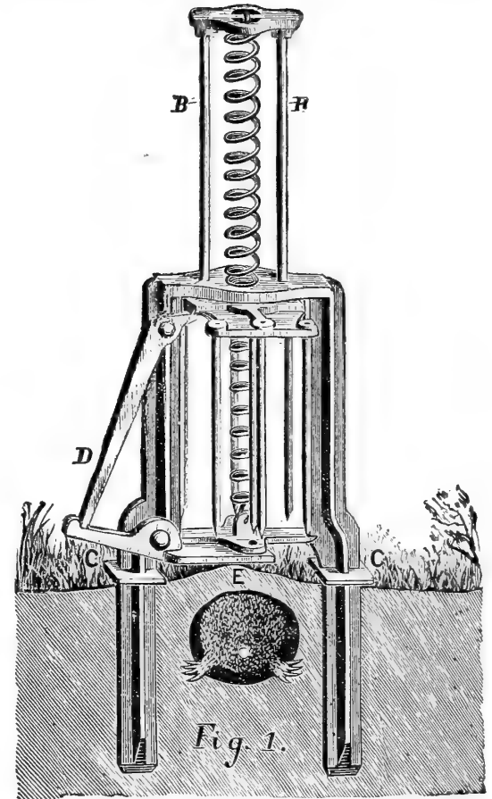
Olmsted Mole Trap.
