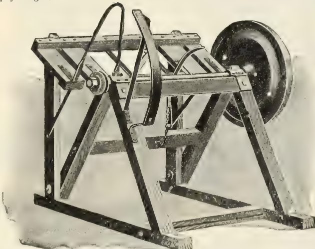
TILTING TABLE WOOD SAW.
