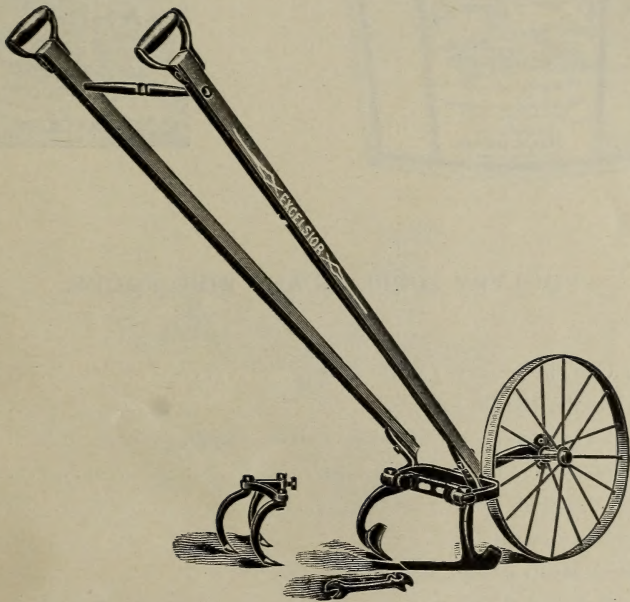
The Excelsior Single Wheel Hoe.
