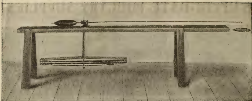
New Cornell Regulator—(Mounted on horse).
