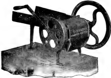
Silver's Clover Cutter.
