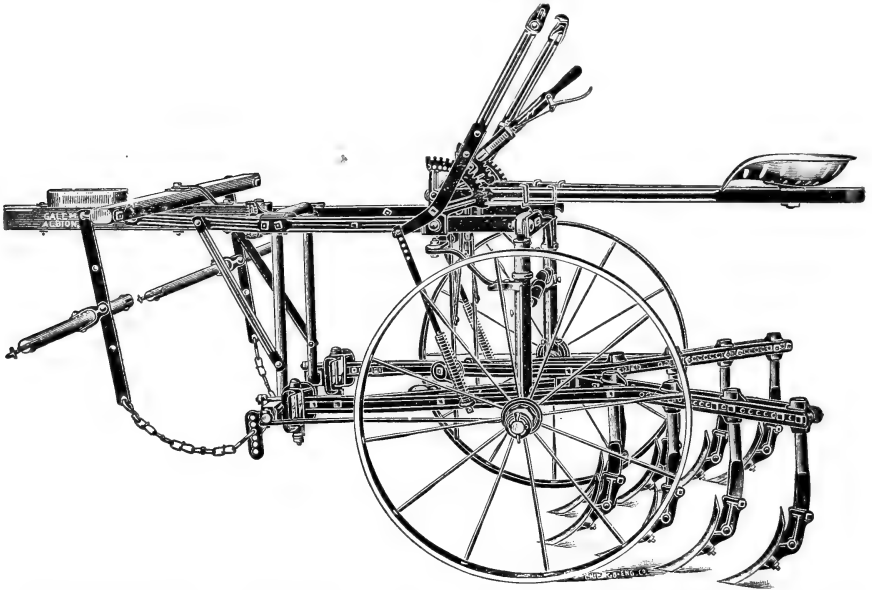
CUT ILLUSTRATES CULTIVATOR FITTED WITH 8 SHOVEL EXTENSION GANGS. WEIGHT 412 POUNDS.
