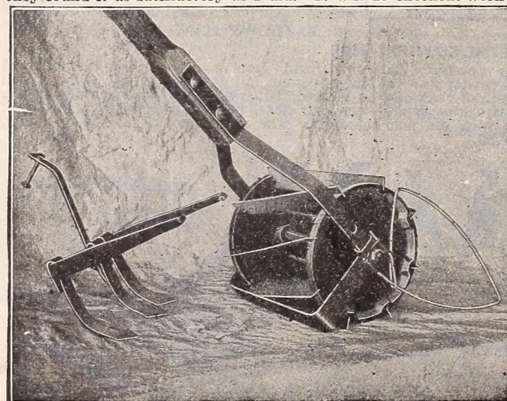
BARKER WEEDER—Back View.
