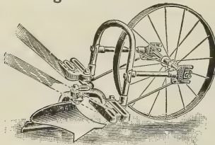
Fig. 82. Price 90c. The Landside Plow Attachment
