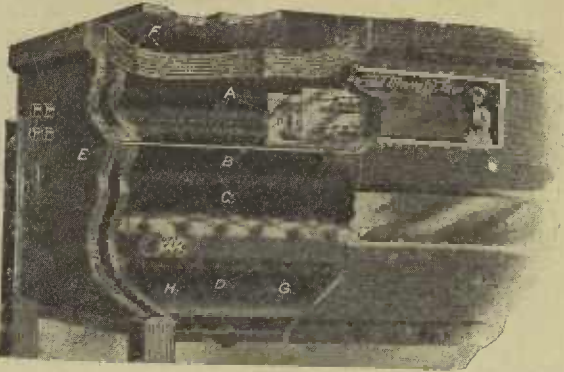
A—Perforated Tubes of heating-chamber. E—Air-tight Diaphragm. B—Inlet Pipe from heater. F—Packing in walls and top. C—Upper Ventilator of egg-chamber. G—Chick-Nursery Bottom. D—Lower Ventilator of egg-chamber. H—Duck-Nursery bottom.
