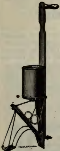
Acme Rotary Corn Planter
