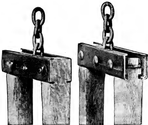
Barnard's Adjustable Steel Head Cattle Stanchion
