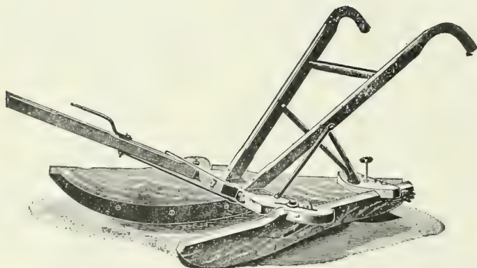
Wood Frame Potato and Pea Coverer
