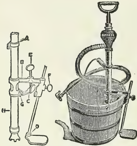
Perfect Success Spray Pump
