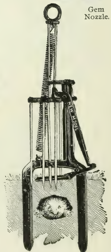
Mole Trap.
