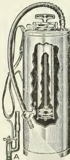
PATENTED. Auto Spray
