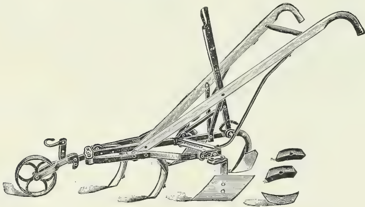
"Triumph" Steel Cultivator and Horse Hoe
