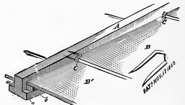
Glazier's Points.
