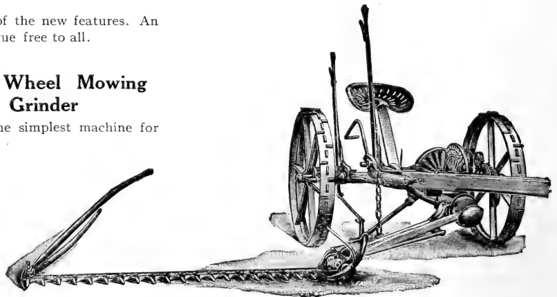
WORCESTER BUCKEYE MOWER
