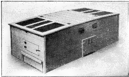
MODEL DOUBLE INDOOR BROODER
