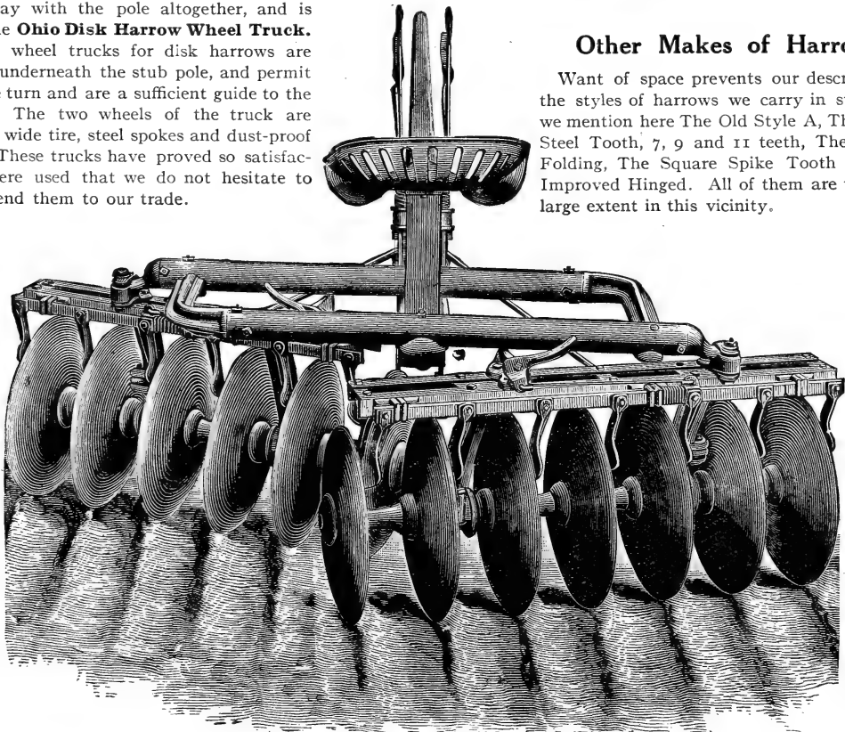
BELL'S CENTER-CUT DISK HARROW
