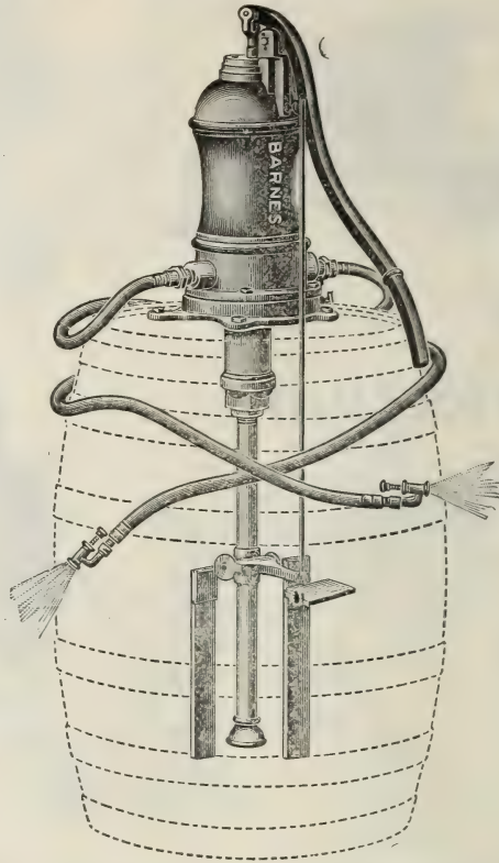
Barnes' New Improved Barrel Spray Pump
