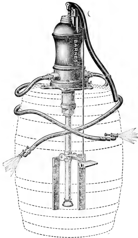
Barnes' New Improved Barrel Spray Pump
