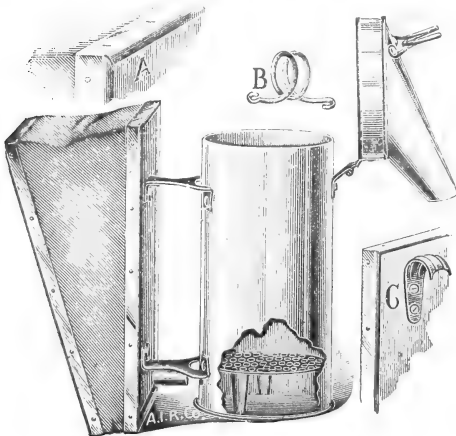
Standard Corneil Smoker
