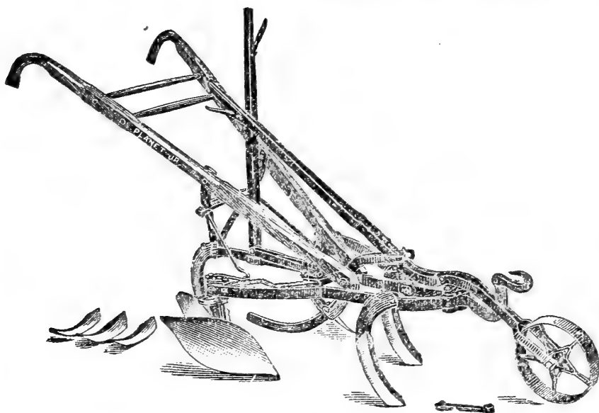
Planet, Jr. Horse Hoe and Cultivator No. 8
