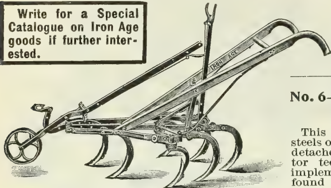
No. 6—Fig. 71, "Iron Age" Horse Hoe as a Cultivator, shown with "Furrow-closing" Attachment
