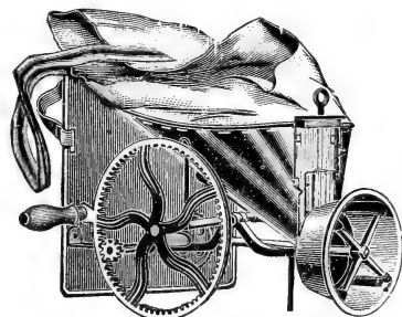
The Cahoon Hand Broadcast Seeder.
