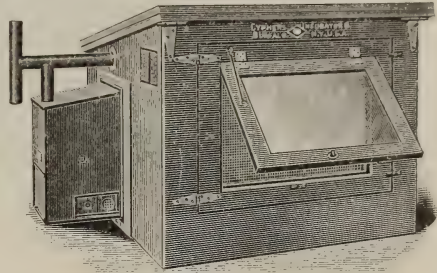
Fig. 3.—Equipped with Cyphers Standard Adaptable Hover, complete. Is self-regulating and self-ventilating. Built throughout of seven-eighths inch thick lumber, including removable floor. Has double door for cleaning and ventilation, single glass window, 12x18 inches, etc., and bears Fire Underwriters' "Inspected Brooder" label.
