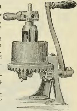
No. 1 CRANK, Weight 30 lbs. Price $5.00.
