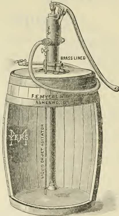
Barrel Spray Pump.
