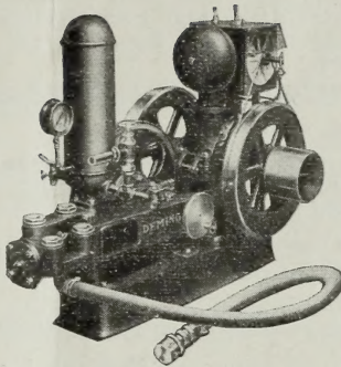
Fig. 656 The "Premier" Power Sprayer for large operation.
