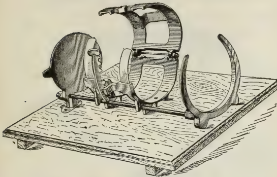
ACME ASPARAGUS BUNCHER, $2.00.
