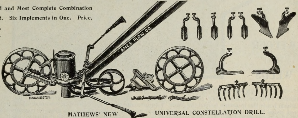
MATHEWS' NEW UNIVERSAL CONSTELLATION DRILL.
