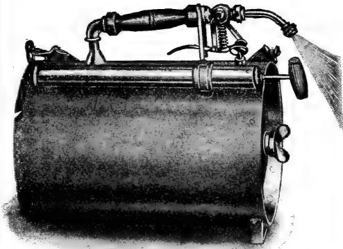
Lowell Fountain Compressed Air Spray.
