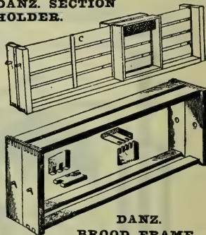
DANZ. SECTION HOLDER.
