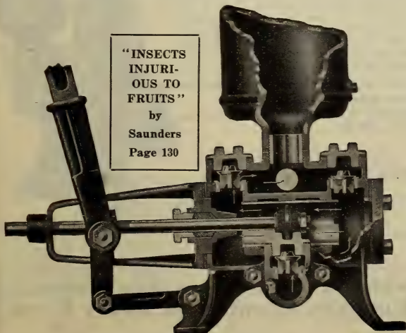
SECTIONAL VIEW OF GOULD'S "ADMIRAL."
