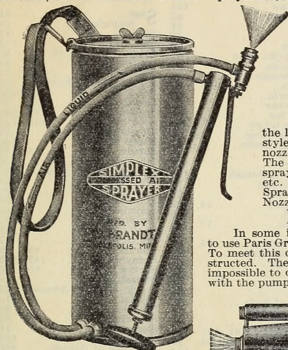
Simplex Sprayer.
