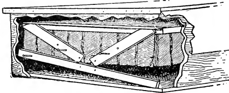
Mandy Lee Fireless—(Showing Inside)
