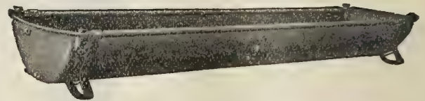
Rivetless Steel Horse and Cattle Troughs. Capacity, 8 gal. per ft. Price, 4 ft., $5.00; 6 ft., $7.25; 8 ft., $9.00.
