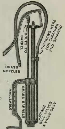
Meyer's Bucket Spray Pump
