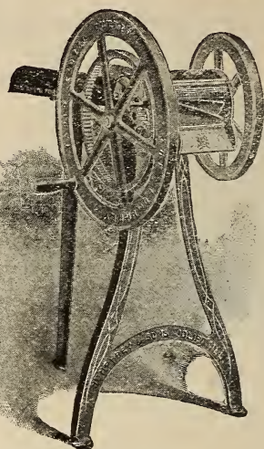
The Humphrey Rapid Clover and Alfalfa Cutter.—A heavy well finished machine to cut clover and alfalfa into pieces 1-8 inch and less. Stand Clover Cutter. (Weight 105 pounds), $11.00.
