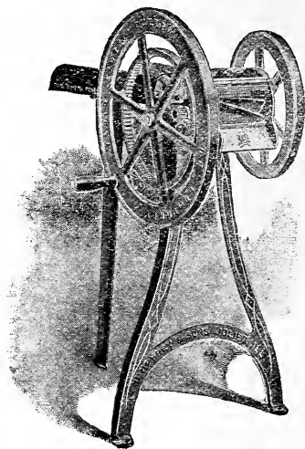
The Humphrey Rapid Clover and Alfalfa Cutter.—A heavy well finished machine to cut clover and alfalfa into pieces 1-8 inch and less. Stand Clover Cutter. (Weight 105 pounds), $11.00.
