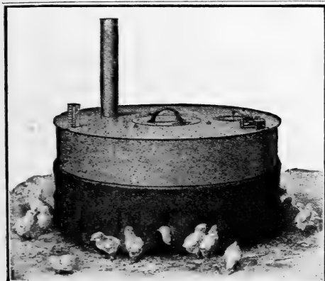
Cyphers New 1913 Portable Hover.
