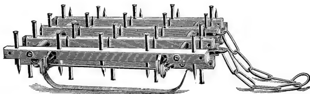
Malta Two-Horse Harrow with 40 Teeth and Runners. (Above cut shows Harrow folded for transportation.)
