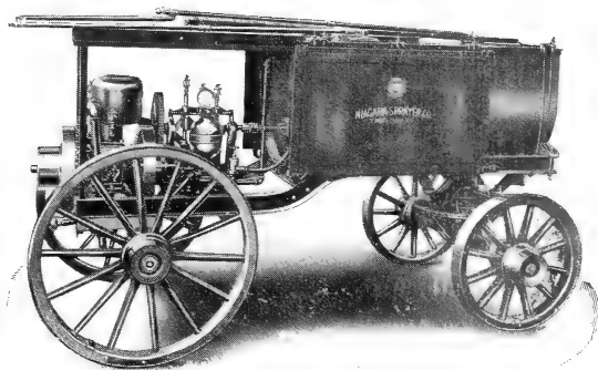
Triplex Outfit with Tower folded.
