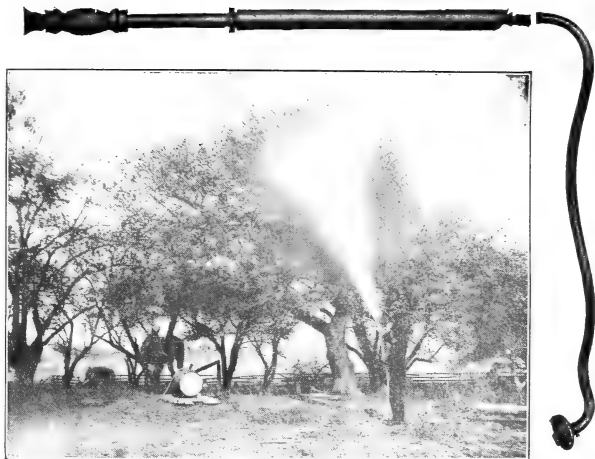
Showing the Standard Pump attached to barrel with 30 feet of hose, enabling the operator to walk around without moving the barrel, covering the entire tree From the Ground without the use of elevated platforms, etc. An ideal orchard sprayer at small cost.
