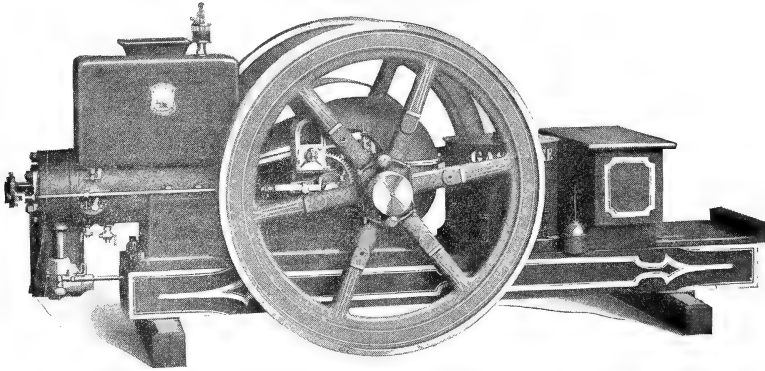
LAUSON FROST KING SEMI-PORTABLE ENGINES.
