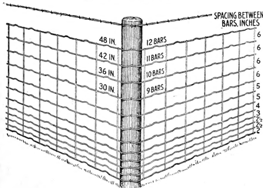
HOG FENCE.
