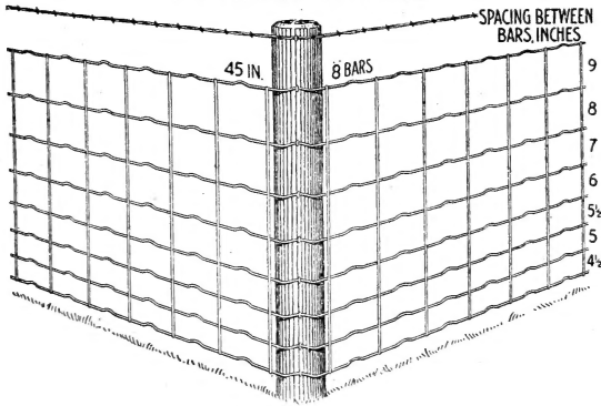
FIELD FENCE.
