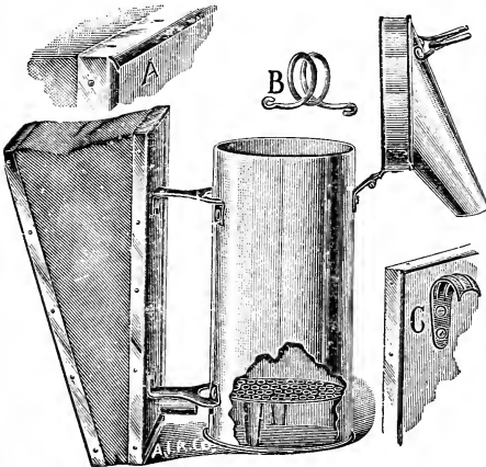
Standard Cornell Smoker
