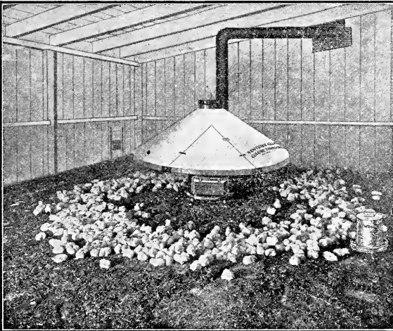
Newtown Giant Colony Brooder
