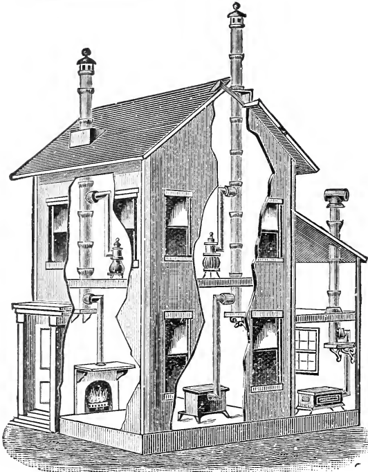
Showing Chimney Tile Put Up
