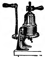
No. 7. Weight 107 Lbs.
