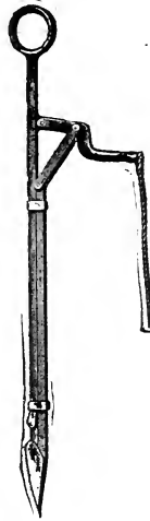
Single Harpoon Horse Pitchfork,
