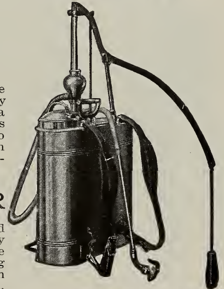
"Success" Knapsack Sprayer.
