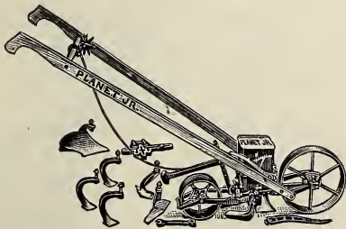
No. 4 Planet Jr. Combined Hill and Drill Seeder, Wheel Hoe, Cultivator, and Plow. Price Complete, $13.25. As a Seeder, only $10.75.
