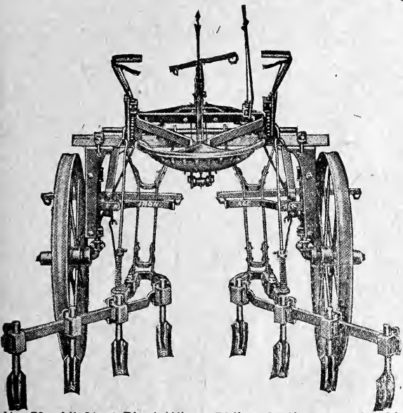
No. 78—All Steel Pivot-Wheel Riding Cultivator. Price $40 No. 76—6-hoe plain, $38.50
