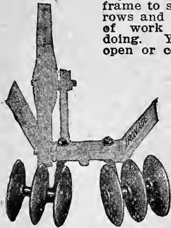
Fig. 369, Disc Cultivating Attachment, $2.50
