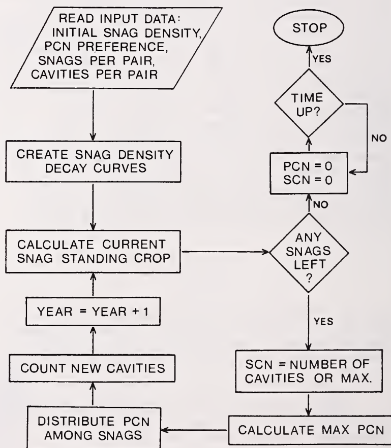
Figure 1.--General flow chart for program CNBIRDS. Data on snag decay rates and use by PCN and SCN are maintained separately for each of 8 snag size and species combinations (see Table 1).
