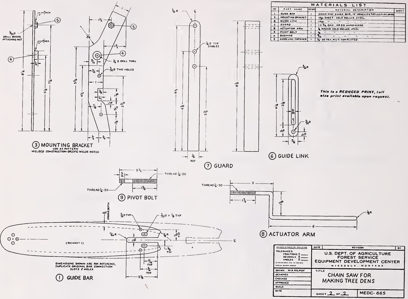
Figure 3B. Modifications to chain saws that are used in constucting cavities: Drawing 2 of 2.
