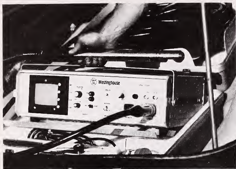
Figure 1.--Westinghouse Miniature Television Camera ETV-1250 control unit and camera with right angle-viewing attachment.
