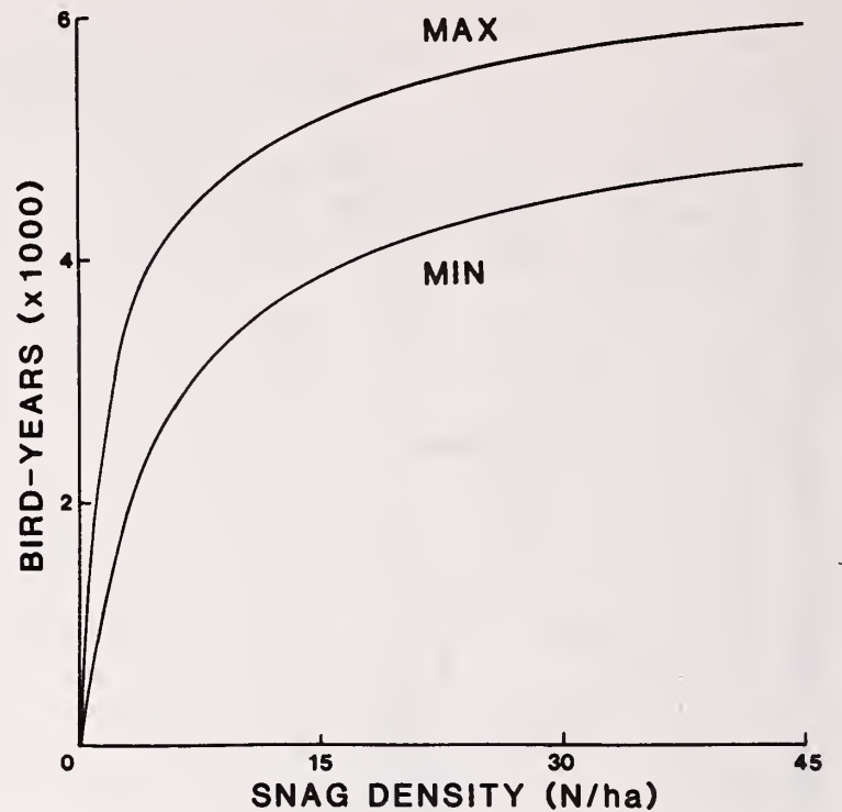
Figure 6.--Simulated response of cavity-nesting birds to changing initial density of snags greater than 38 cm dbh. The upper curve (max) was computed assuming that each pair of PCN requires 15 snags and excavates 3 cavities per year; the lower curve (min) assumes 48 snags per pair and 1 cavity.
