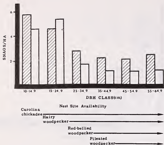
Figure 2.--Distribution of snags by diameter class on TSI'ed (cross-hatched) and non-TSI'ed (open bars) watersheds, Breathitt County, Kentucky, 1981, 20 years post-treatment. Nest site availability is also depicted for four common primary cavity-nesters.
