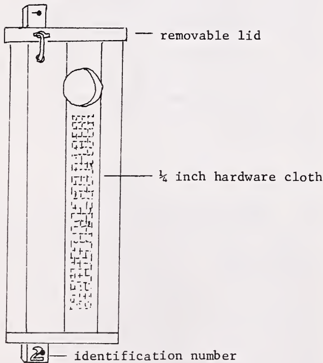
Figure 1.--Coppery-tailed trogon nest box.
