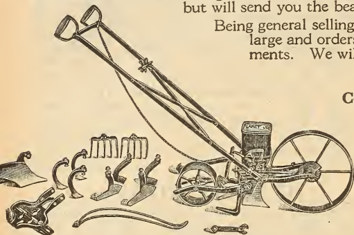
No. 28—Combined Hill and Drill Seeder.
