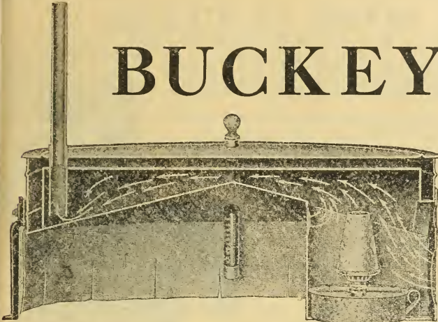
Showing a Sectional View of the "Buckeye" Brooder
