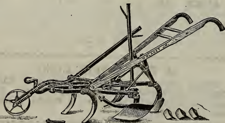
No. 3 Planet Jr. Horse Hoe and Cultivator.
