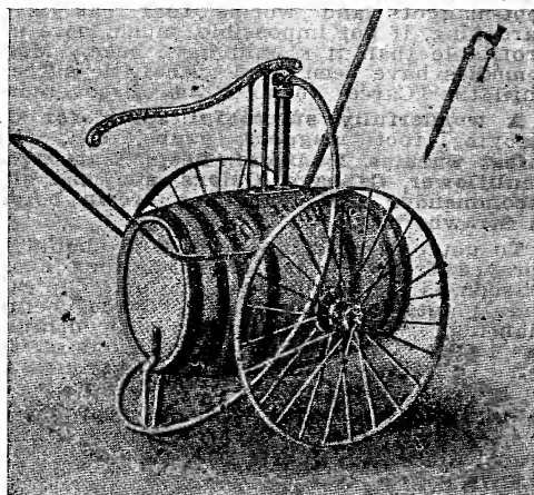
Hardie Wheel Outfit No. 21
