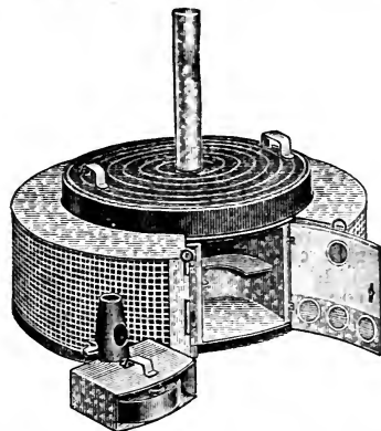
Economy Hover with rat-proof wire cage; showing construction of lamp, lamp box and lamp slide.
