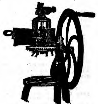
Mann's No. 7 for green bone.
