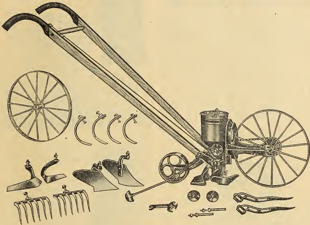
No. 1 Blocki Hill and Drill Seeder
