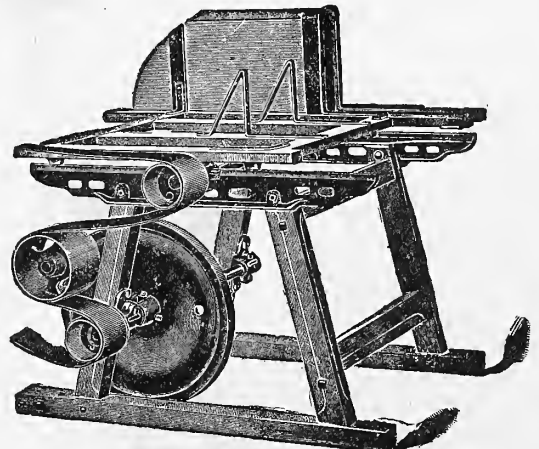
SLIDING TABLE POLE SAW
