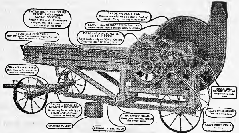
Showing Machine Mounted Special Features of No. 40, No. 60 and No. 90
