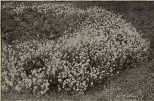
Alyssum, Carpet-of-Snow
