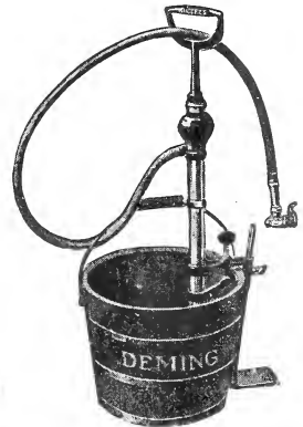
Fig. 689. "Perfect Success" Bucket Spray Pump (Bucket not furnished)
