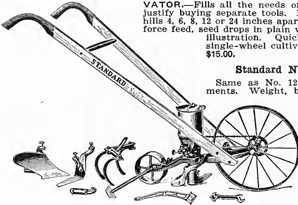
Standard No. 12 Hill and Drill Seeder and Cultivator
