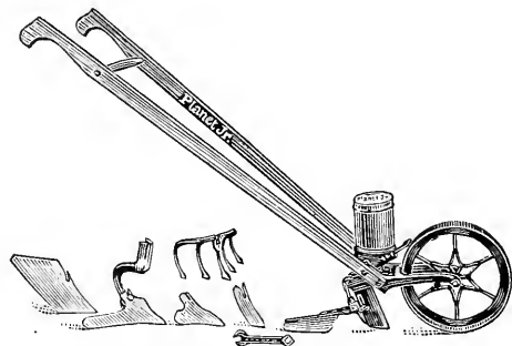
No. 31 Planet Jr. Combined Drill Seeder Single Wheel Hoe.
