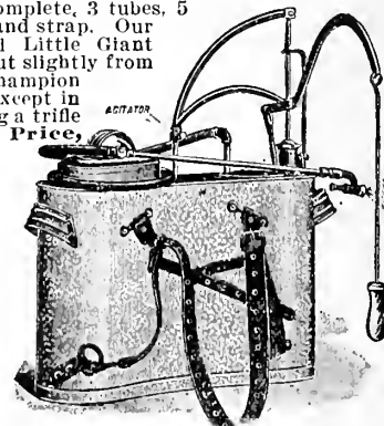
The Garfield Knapsack Sprayer
